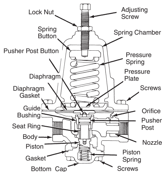
Type G-60 Interior Steam Regulator
